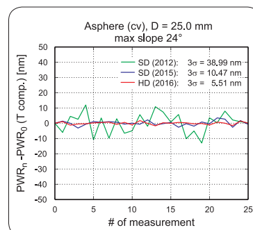
Asphere (cv), D = 25.0 mm, max slope 24°
